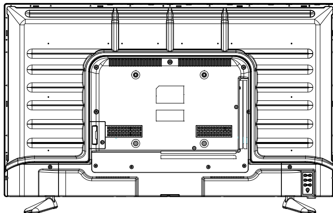
TV1 (S2) TV2 (T2/C) HDMI3 OPTICAL Common Interface USB 5V --- 500mA
