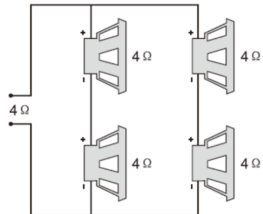
Series/parallel wiring
