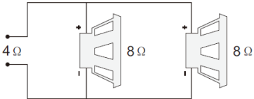
Parallel wiring
