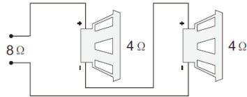
Series wiring
