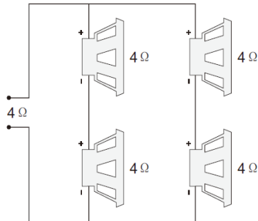
Series/parallel wiring
